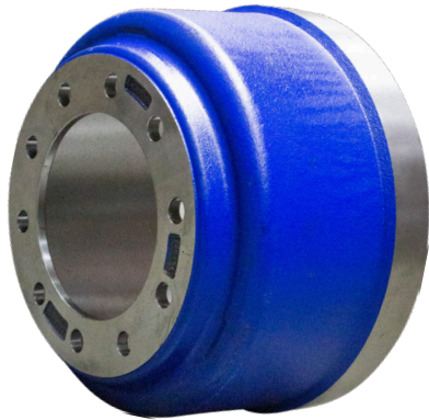
Drive Brake Drum Item no. 09078 UPC 6-59806-09078-6
