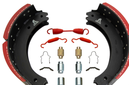
Premium Brake Shoe Kit 4711 Item no. 09650 UPC 6-59806-09650-4
